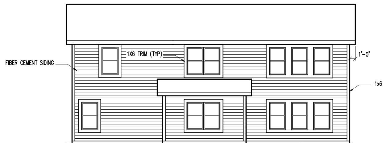
REAR ELEVATION. . . .3/32"
