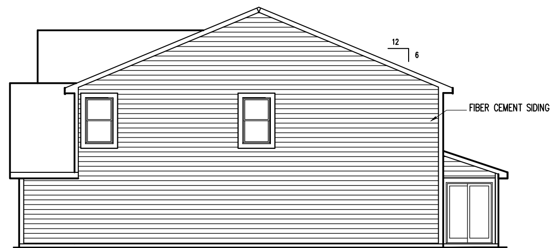
RIGHT ELEVATION. . . .3/32"
