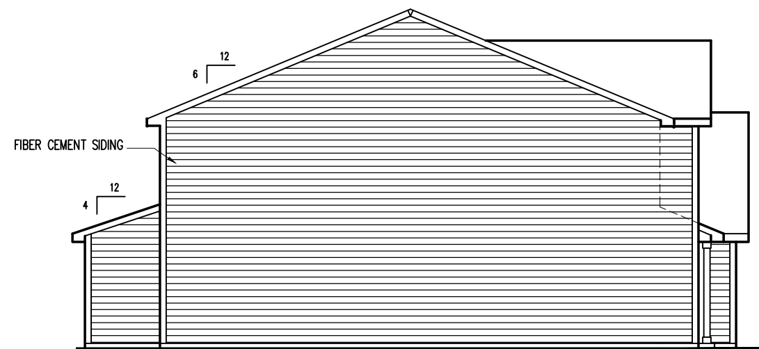
LEFT ELEVATION. . . .3/32"
