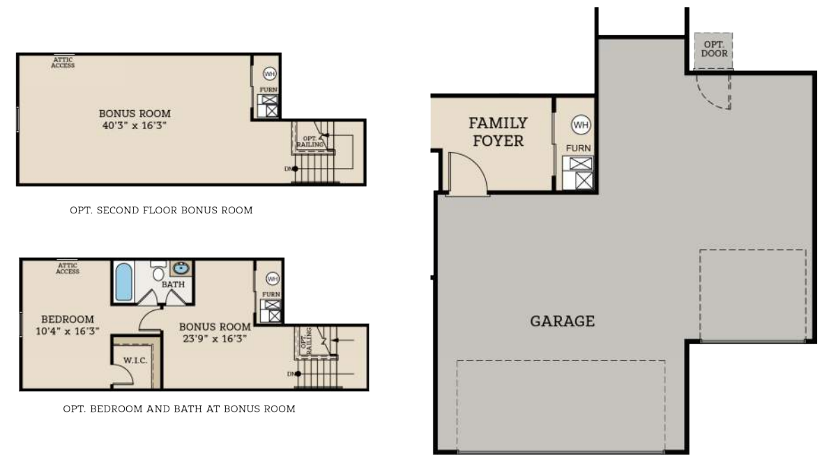
OPT. 3 CAR GARAGE
