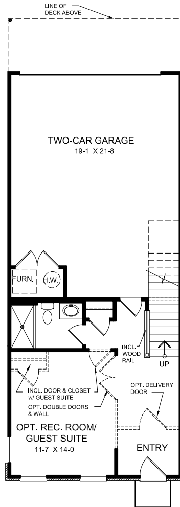
OPT. FINISHED LOWER LEVEL REC. RM/ OPT. GUEST SUITE w/ FULL BATH
