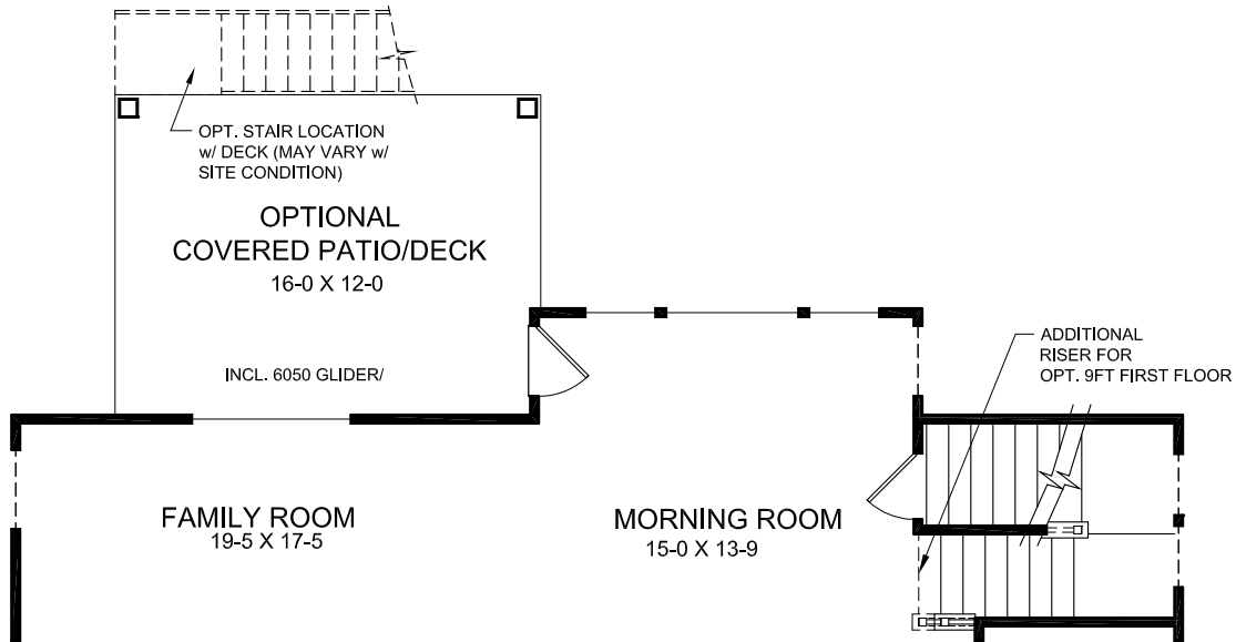
OPTIONAL COVERED PATIO/DECK
