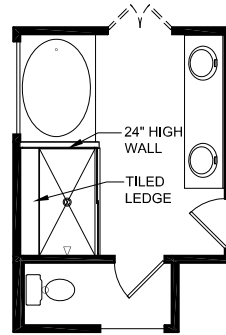
OPTIONAL DELUXE GARDEN BATH
