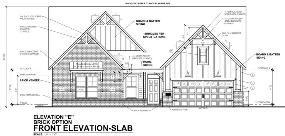
Elevation E Opt. Brick
