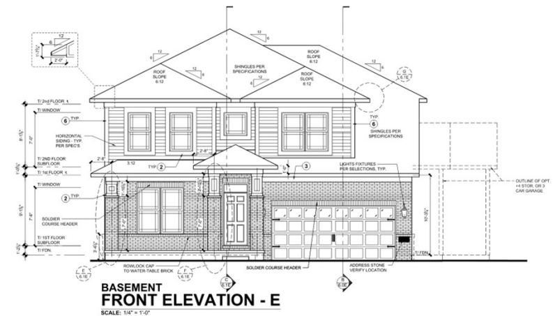
Elevation E Opt. Brick
