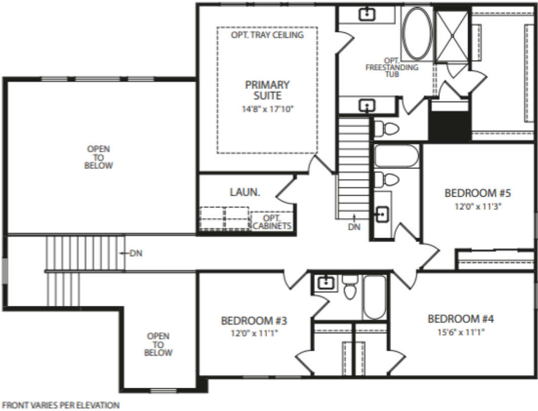
Second Level
