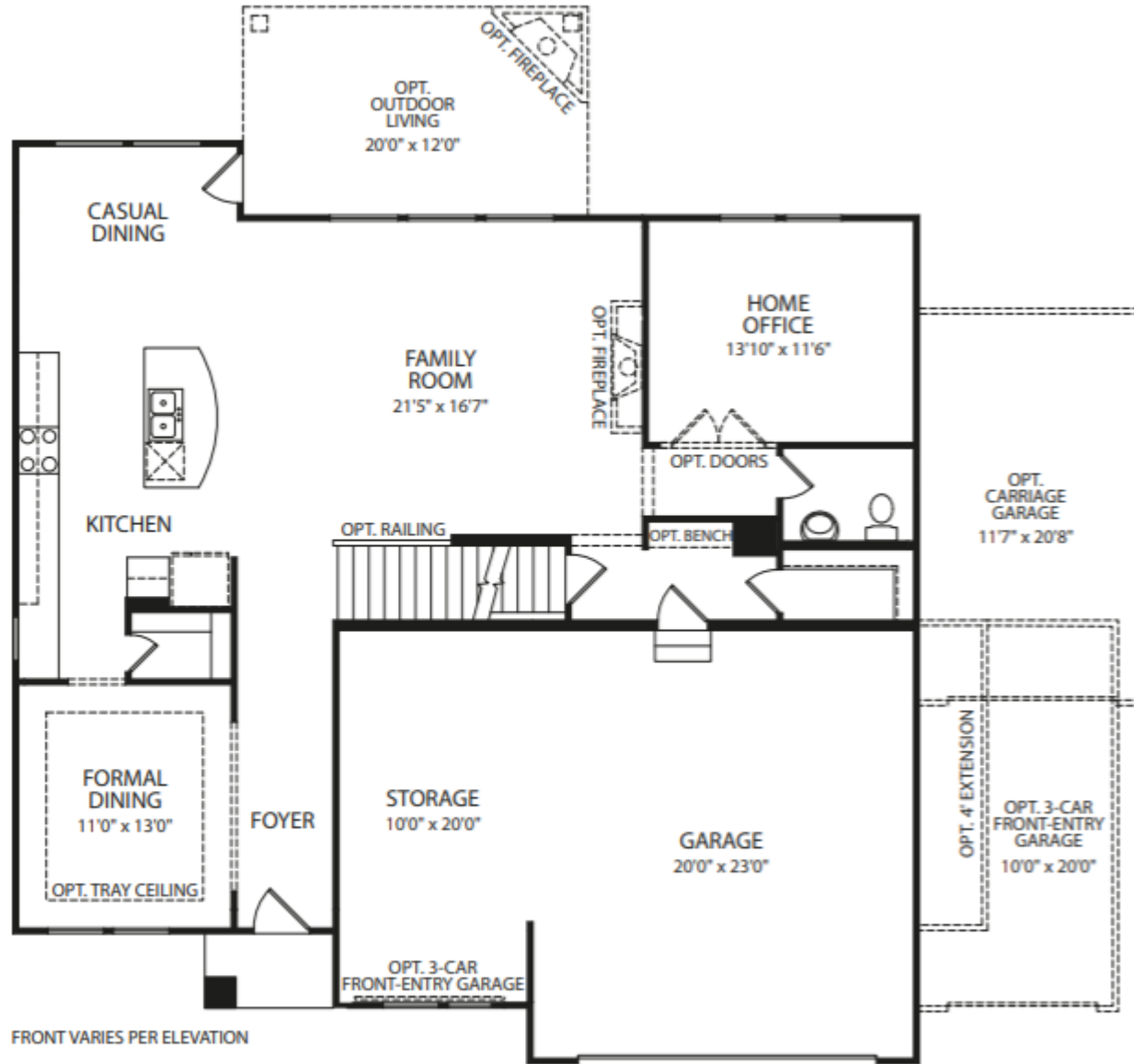
Main Level
