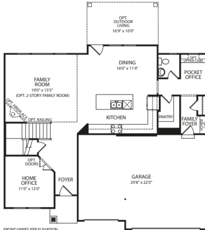
Main Level
