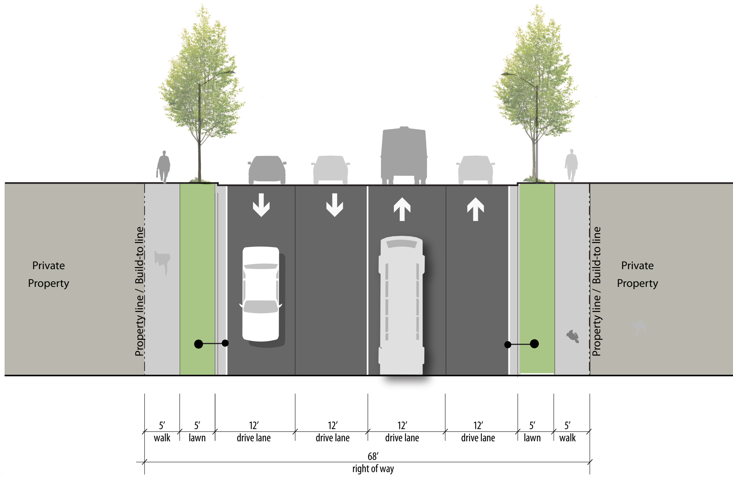
TYPICAL STREET SECTION
