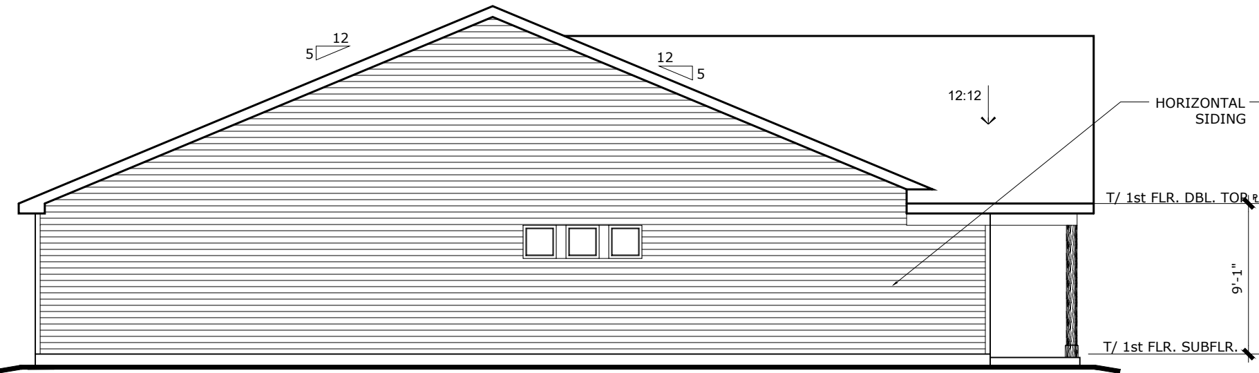
LEFT ELEVATION
