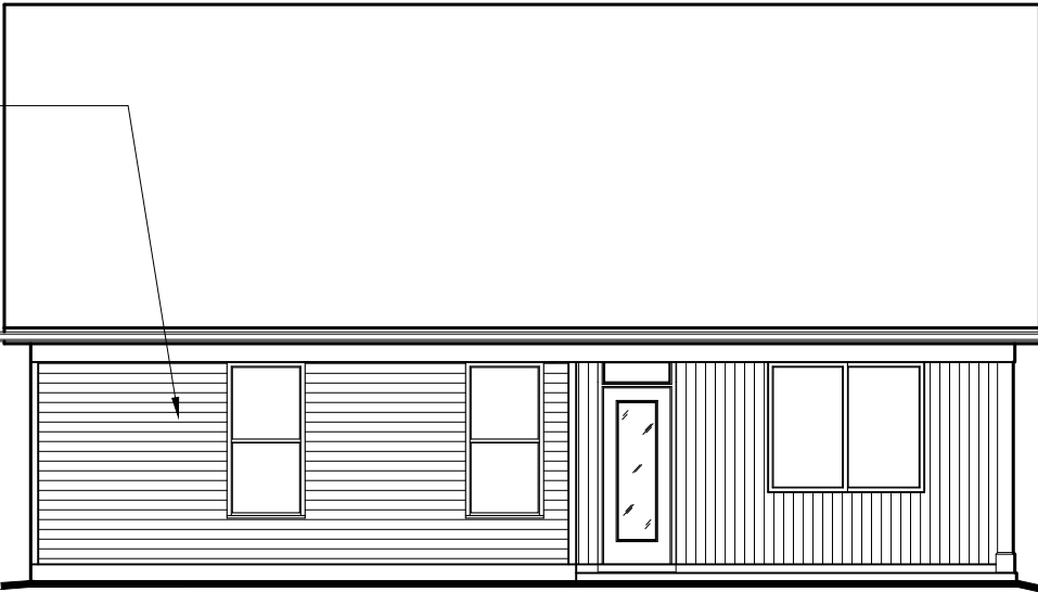
REAR ELEVATION
