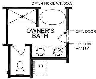
OPT. OWNER'S BATH w/ SEPARATE SHOWER & GARDEN TUB
