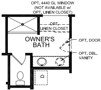
OPT. 5FT SHOWER IN LIEU OF INCLUDED OF TUB
