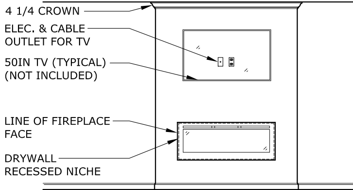
OPTIONAL WALL-MOUNT ELECTRIC FIREPLACE #1 SHOWN w/ INCLUDED 8FT FIRST FLR CEILING HEIGHT
