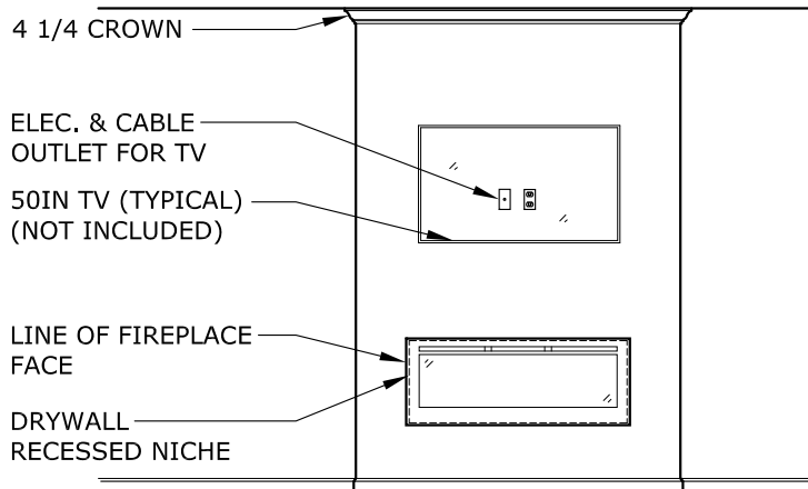
OPTIONAL WALL-MOUNT ELECTRIC FIREPLACE #1 SHOWN w/ OPTIONAL 9FT FIRST FLR CEILING HEIGHT
